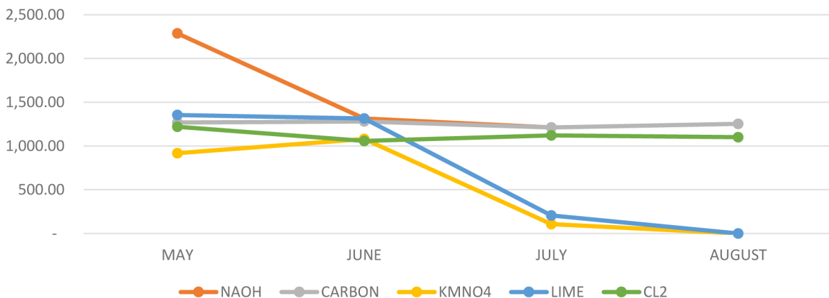
Chemical Reduction After AO3 Solutions Installed Water Intake Aeration System
